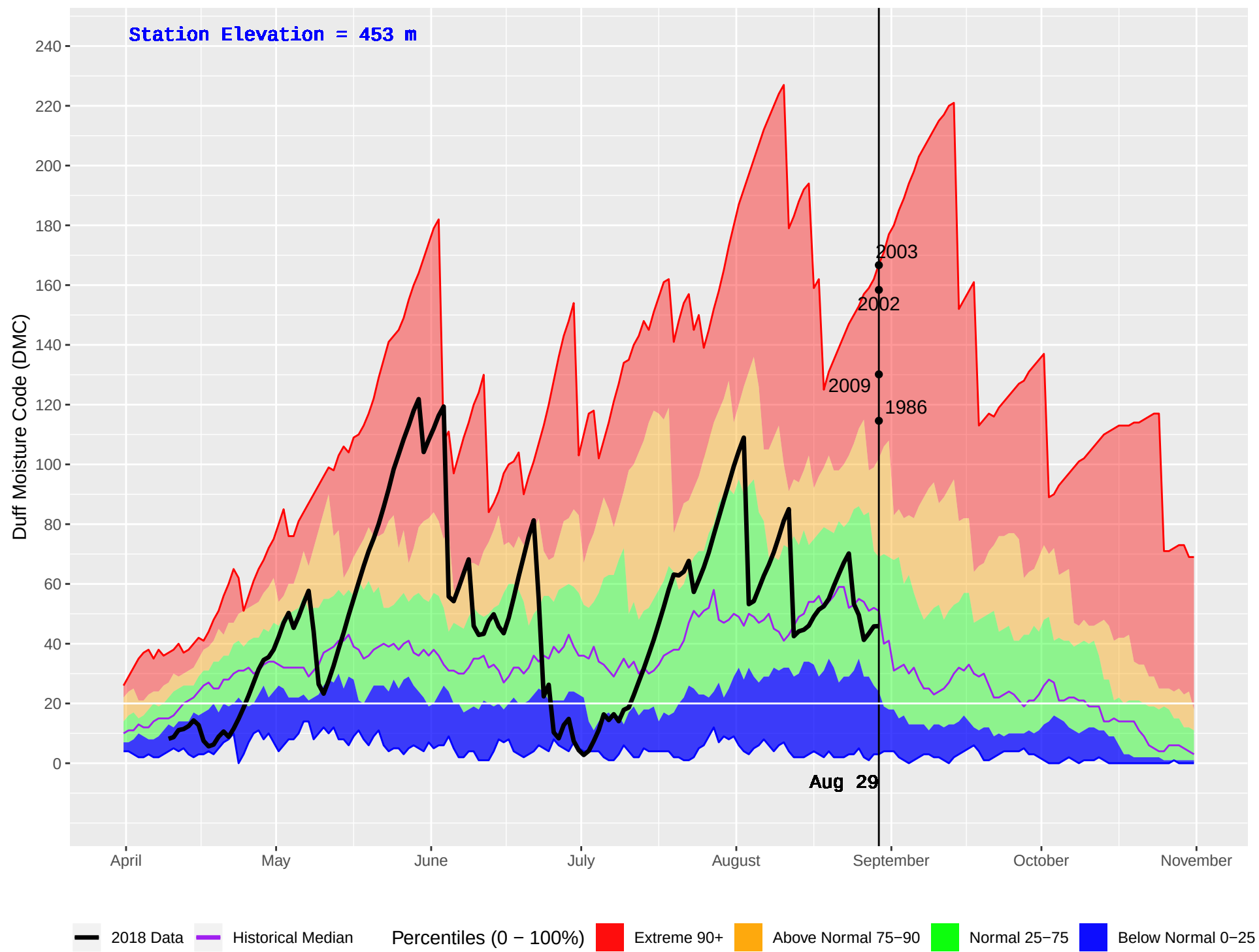
CLEARWATER HUB (239) : Historical (1976–2016) and Current (2018) Daily Duff Moisture Code (DMC)
